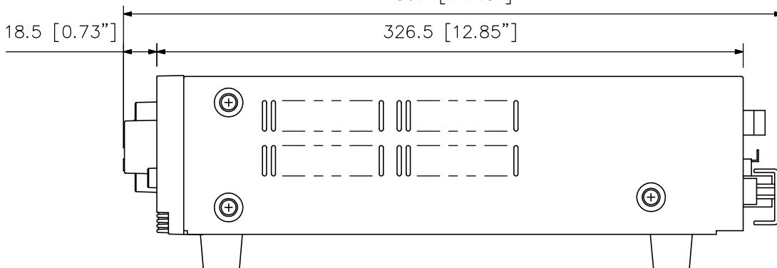
Side View
