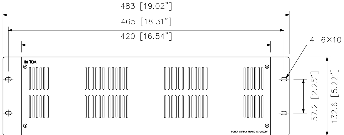
Front View
