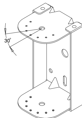
[Wall bracket]
